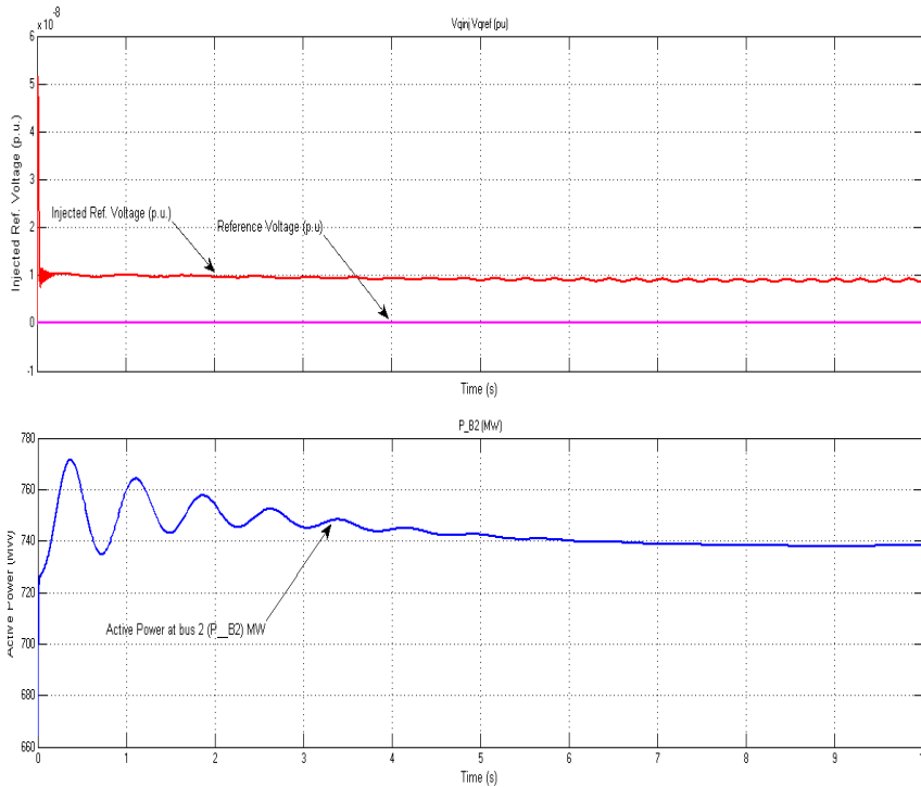
Figure.6 Test System Without SSSC
