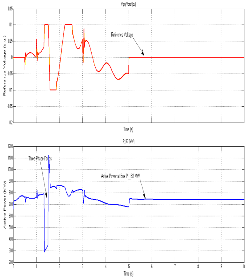
Figure.12 the Effect of POD controller on test system operation
