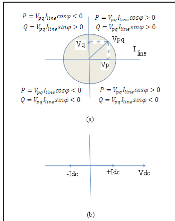
Figure.1 Phasor Diagram of the SSSC Operation
