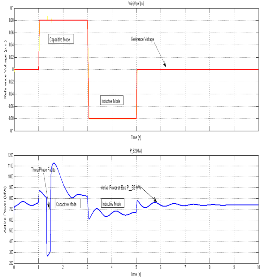
Figure.11 Test system subjected to three-phase faults
