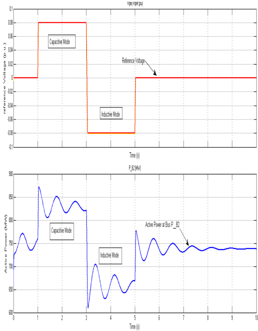
Figure.10 Operation of test system with the reference voltage V_{qref} .
