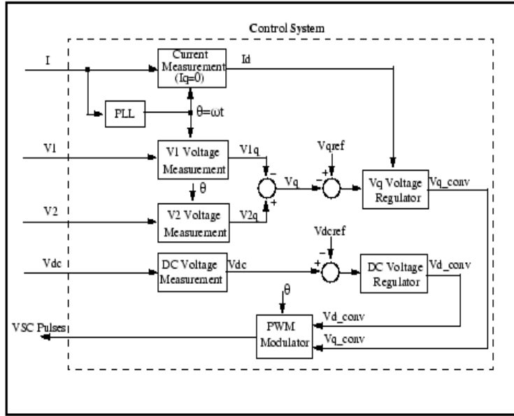
Figure.5, SSSC control system implementation
