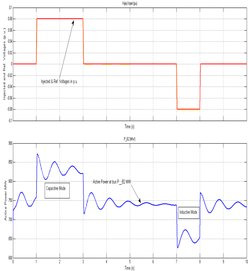
Figure.8 Test System Without POD Controller
